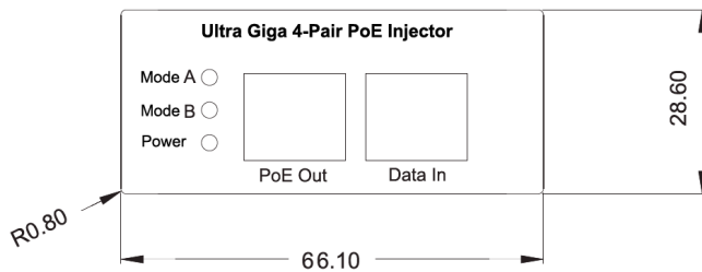
Front Panel
